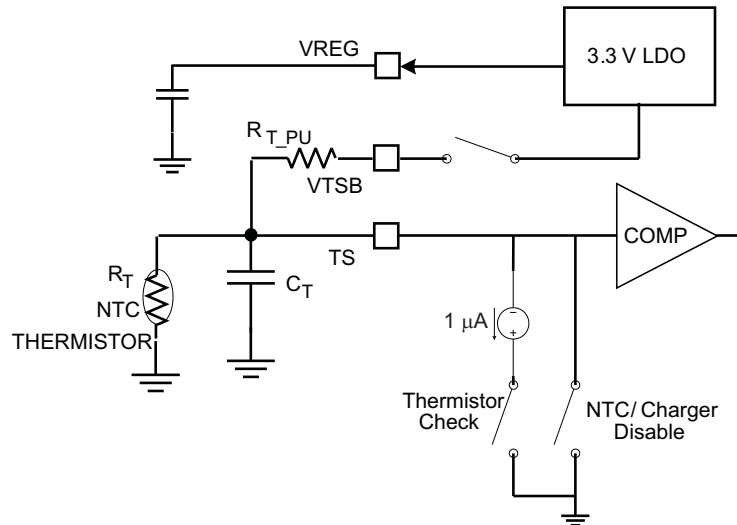
Figure 12. TS and VTSB Pin Interface
