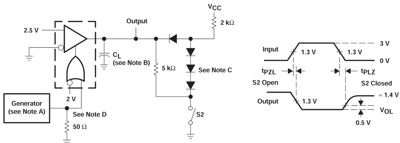
TEST CIRCUIT
