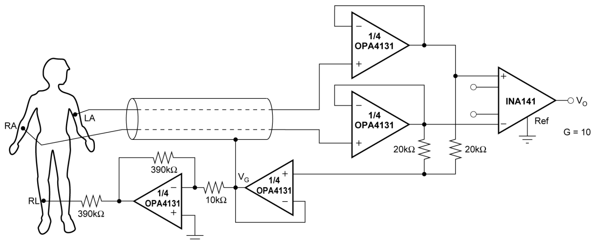
Figure 7-4. ECG Amplifier With Right-Leg Drive
