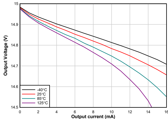
Figure 6-12. Positive Output Voltage Swing vs Output Current
