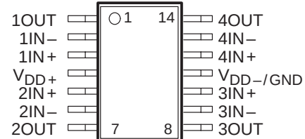
TLV2334 PW PACKAGE (TOP VIEW)
