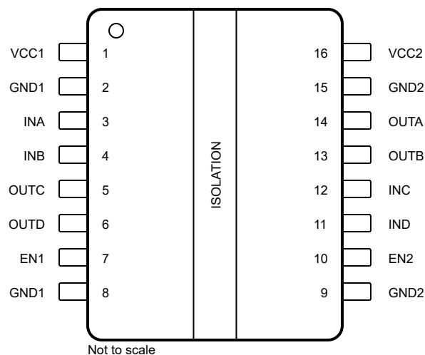
Figure 4-3. ISO6542-Q1 and ISO6542F-Q1 Top View
