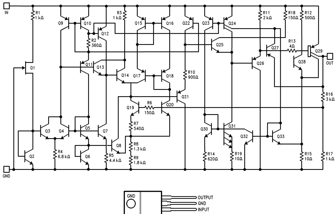
Figure 1. (TO-220)
