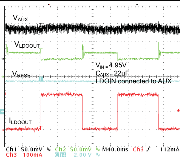
Figure 15. LDO Load Transient Response 0 mA - 200 mA
