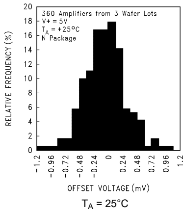
Figure 5-1. Distribution of LMC6082 Input Offset Voltage
