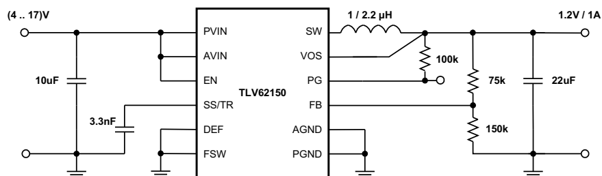
Figure 44. 1.2-V/1-A Power Supply
