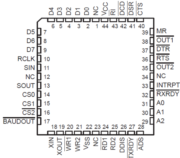
Figure 4-2. FN Package (Top View)
