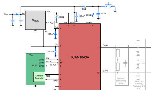
Simplified Schematic
