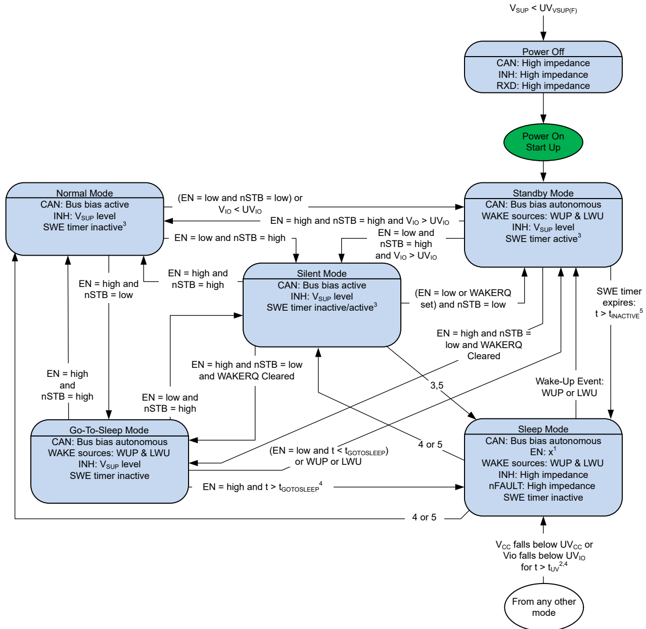
Figure 7-4. TCAN1043A-Q1 State Machine
