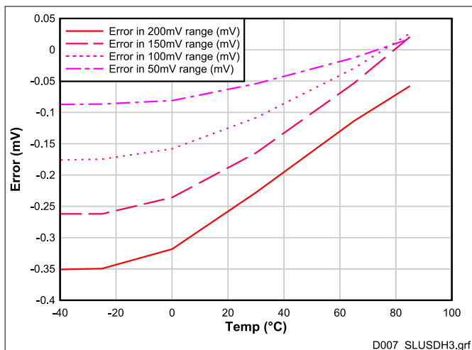
Figure 7-10. Current Measurement Error vs. Temperature
