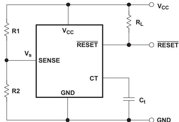
Figure 18. Setting the Sense Voltage
