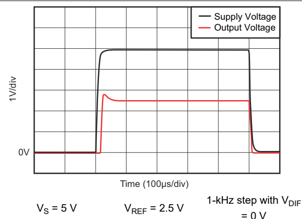
Figure 5-21. Start-Up Response
