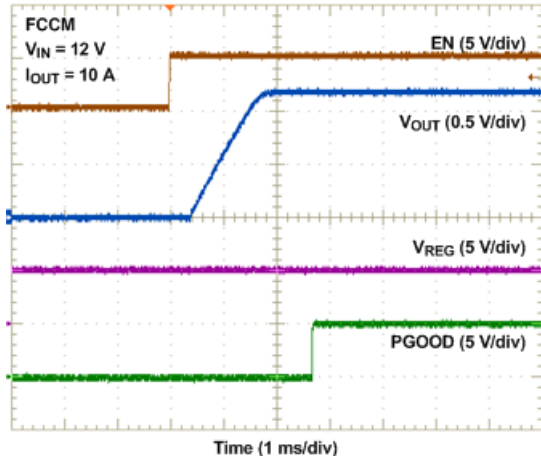
Figure 9-2. Start-Up
