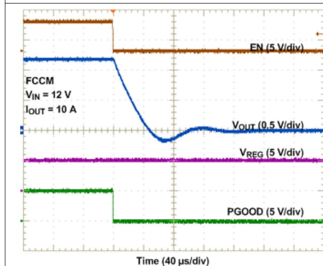
Figure 9-15. Shutdown
