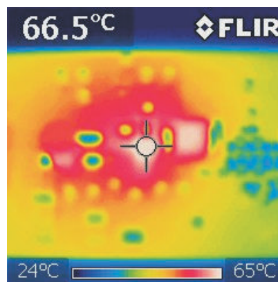
Figure 9-9. Overtemperature Protection
