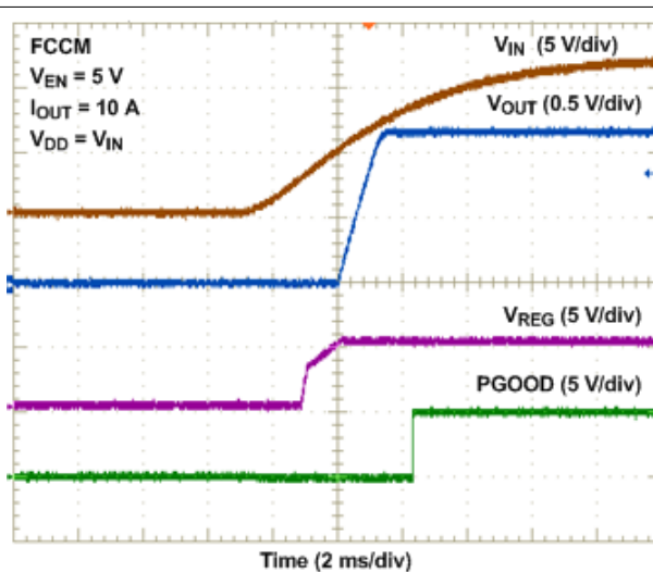
Figure 9-16. UVLO Start-Up
