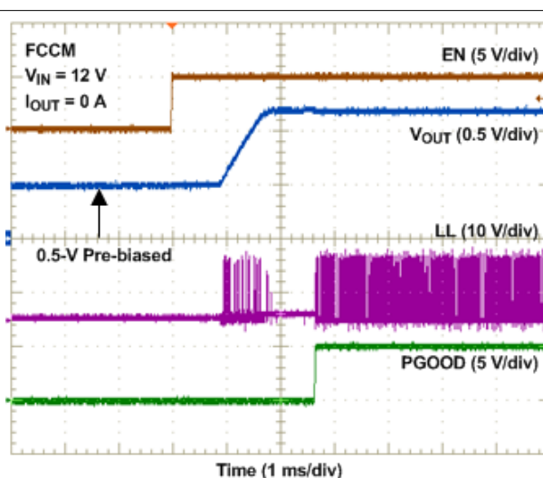
Figure 9-14. Pre-Bias Start-Up
