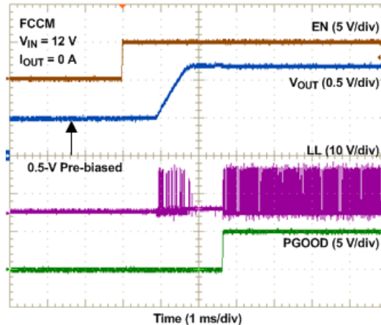
Figure 9-3. Pre-Bias Start-Up
