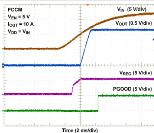
Figure 9-5. UVLO Start-Up
