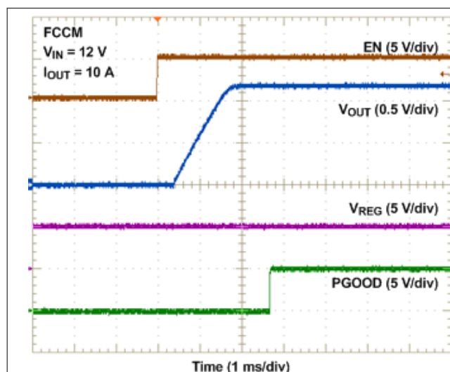
Figure 9-13. Start-Up
