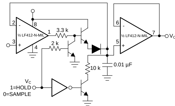
Figure 29. Single-Supply Sample and Hold
