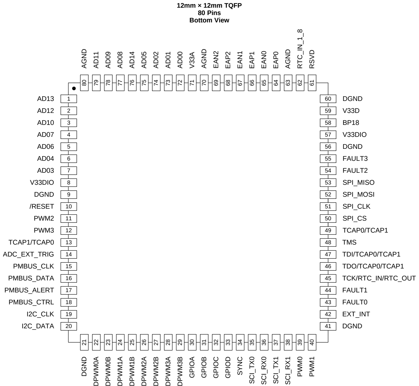
Pin Functions
