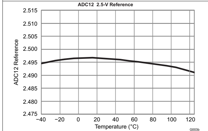
Figure 6. ADC12 2.5-V Reference vs. Temperature
