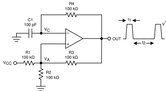
Figure 8-9. Square-Wave Oscillator
