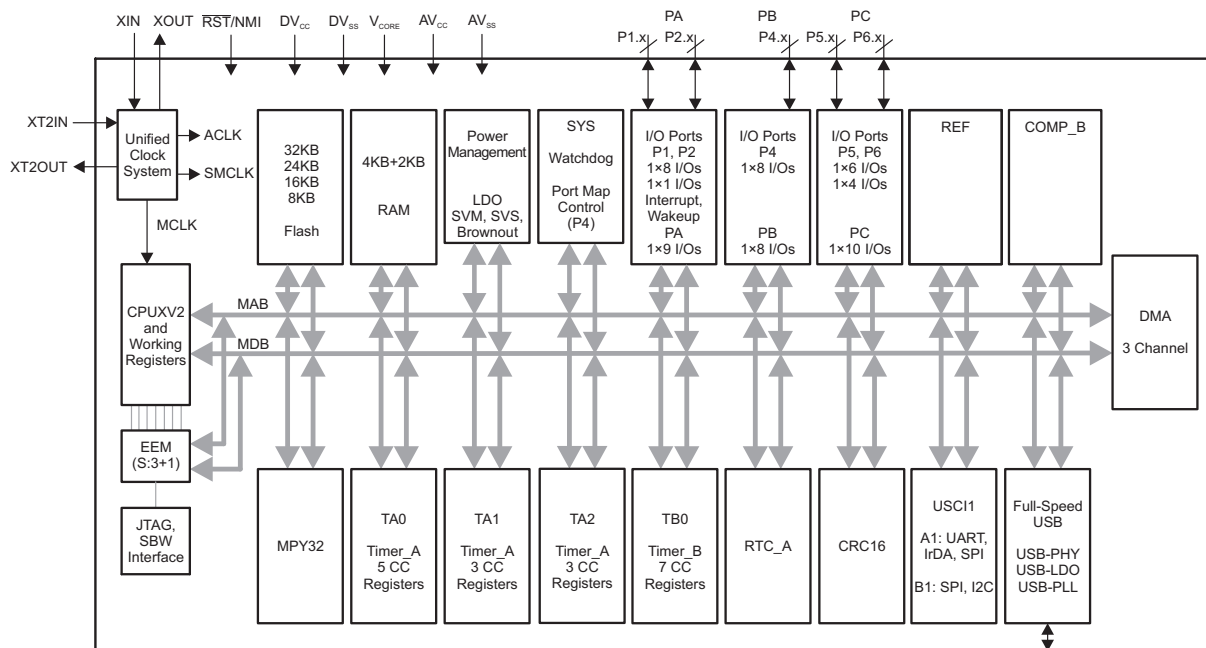
Figure 1-4. Functional Block Diagram – RGZ Package – MSP430F5503, MSP430F5502, MSP430F5501, MSP430F5500
