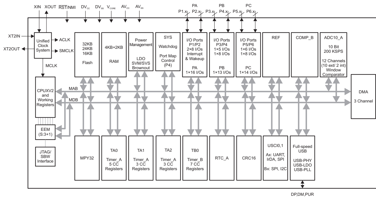
Figure 1-1. Functional Block Diagram – RGC, ZXH, or ZQE Package – MSP430F5510, MSP430F5509, MSP430F5508
