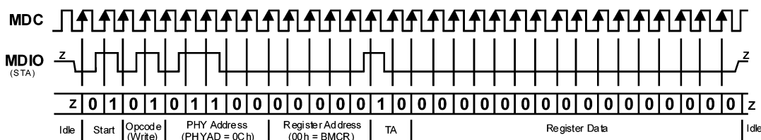
Figure 5-3. Typical MDC/MDIO Write Operation
