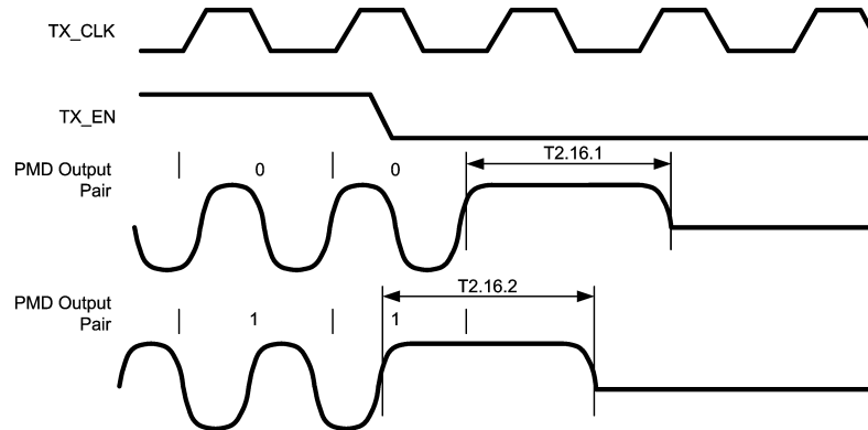
Figure 4-14. 10BASE-T Transmit Timing (End of Packet)
