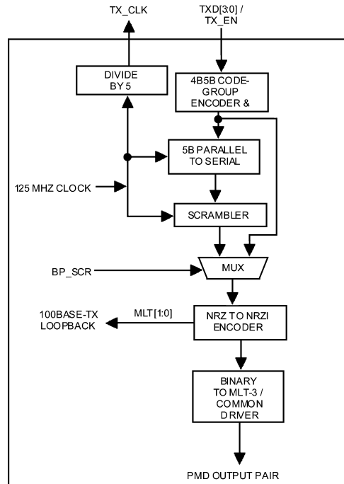
Figure 5-5. 100BASE-TX Transmit Block Diagram
