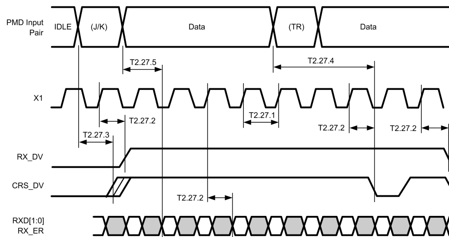
Figure 4-25. RMI Receive Timing
