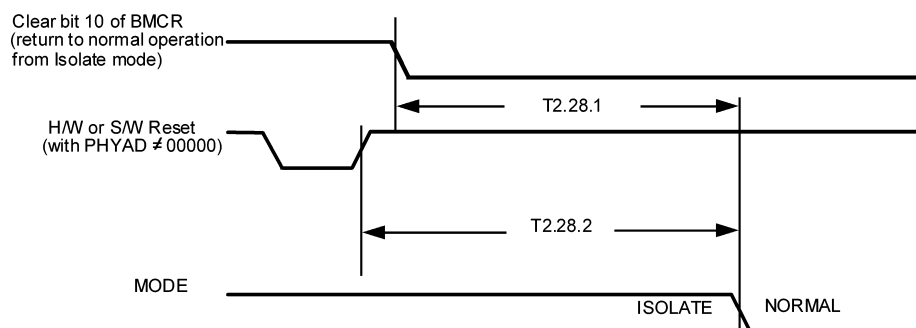
Figure 4-26. Isolation Timing
