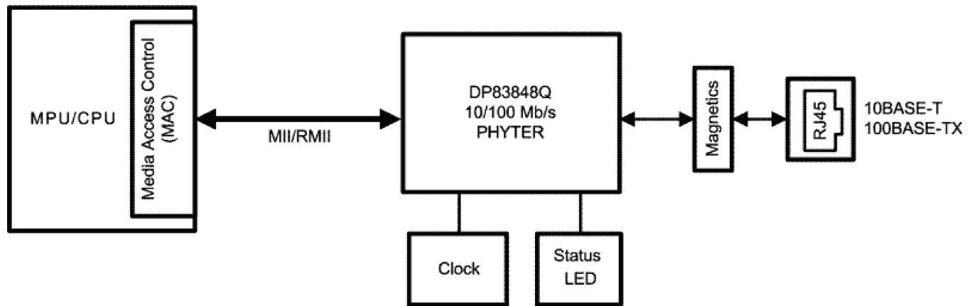
Figure 6-1. Typical Application
