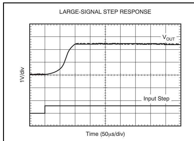
Figure 32. DAC1280 Large-Signal Step Response (Noise Removed for Clarity)
