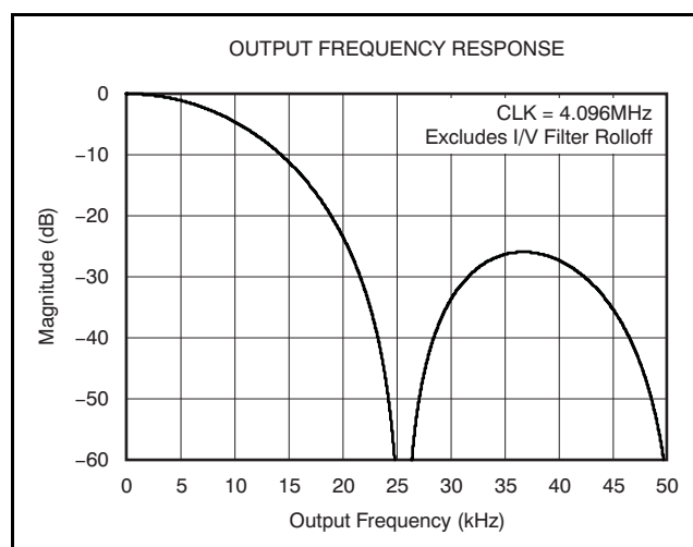
Figure 33. Output Frequency Response
