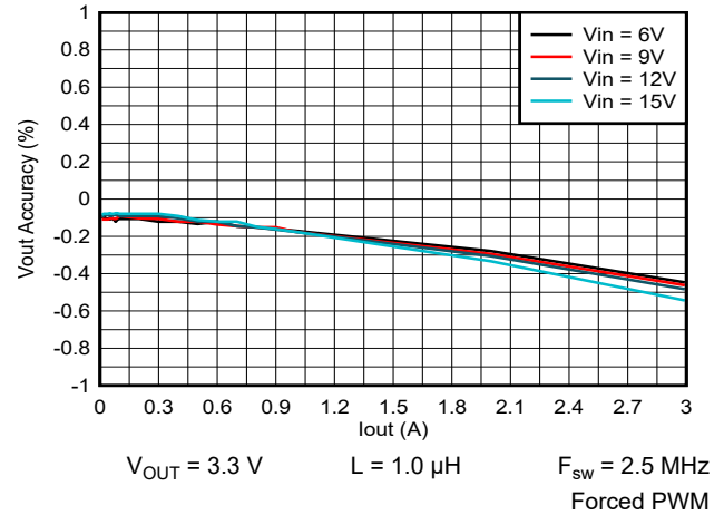
Figure 9-57. Output Voltage vs Output Current
