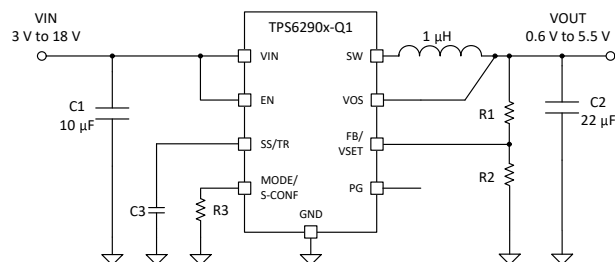
Simplified Schematic
