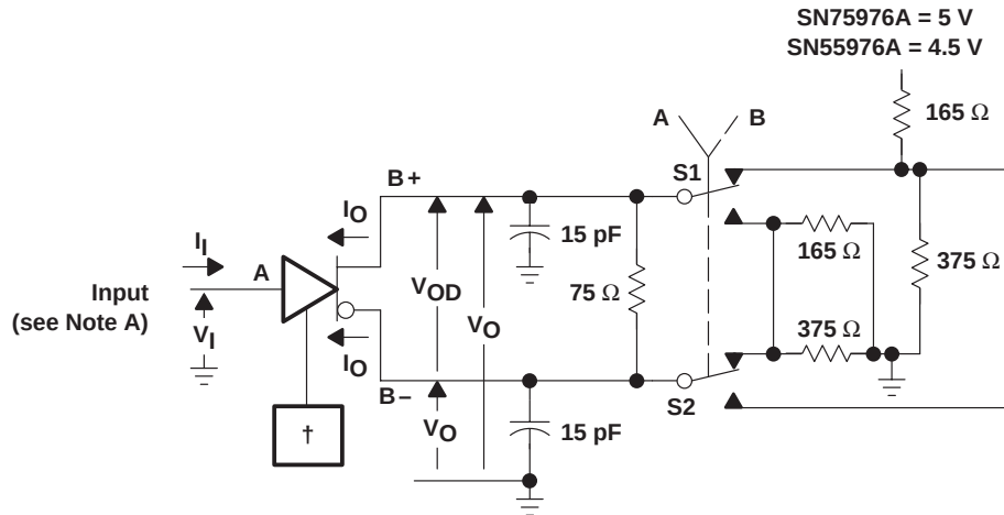
Figure 1. Driver Test Circuit, Currents, and Voltages \ddagger
