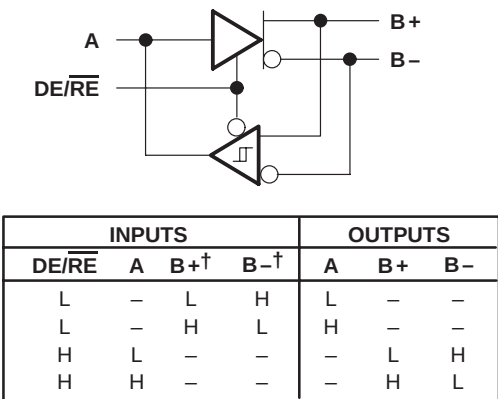
TRANSCEIVER
