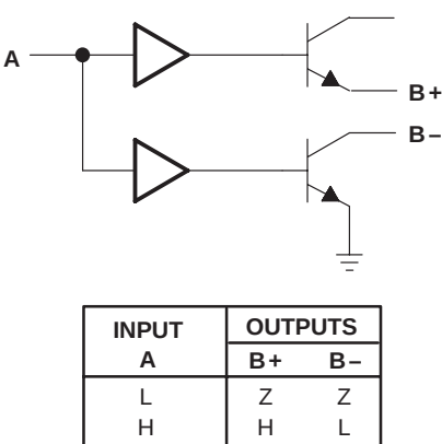
WIRED-OR DRIVER
