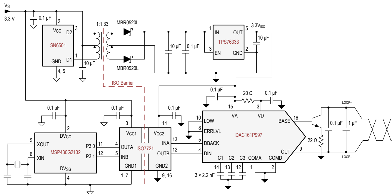
Figure 9-1. Isolated 4-mA to 20-mA Current Loop
