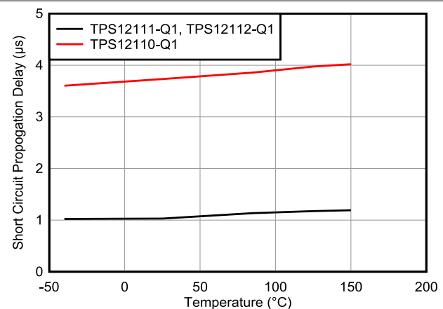
Figure 6-12. Short Circuit Protection Response Time ( t_{SC} ) vs Temperature
