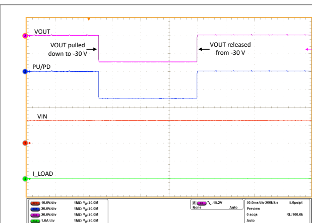
Figure 8-17. Output Short to -30 V Response with VIN = 12 V and INP = LOW
