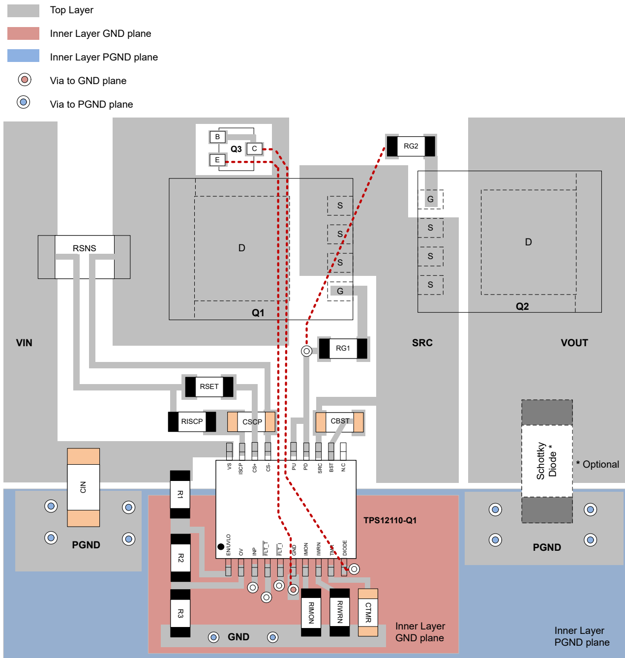
Figure 9-17. Typical PCB Layout Example for TPS12110-Q1 With B2B MOSFETs
