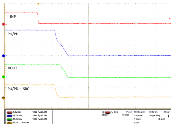
Figure 9-5. Turn-OFF Response of TPS1211-Q1 for INP -> HIGH to LOW and C_{BST} = 470 nF
