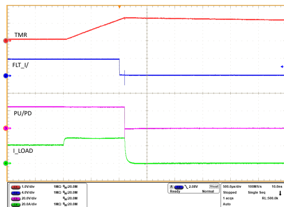
Figure 9-7. Overcurrent Response of TPS1211-Q1 for a Load Step from 20 A to 32 A with 30-A Overcurrent Protection Setting
