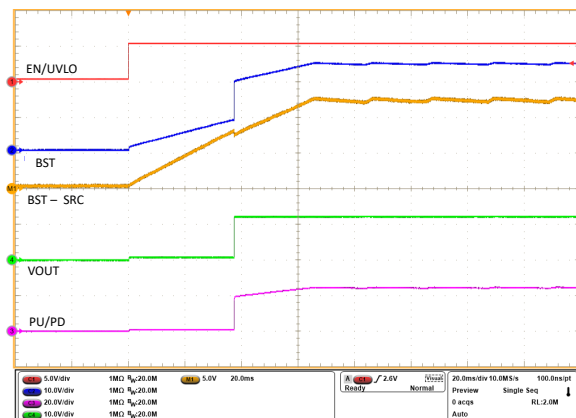
Figure 9-3. Start-Up Profile of Bootstrap Voltage for INP = HIGH and C_{BST} = 470 nF
