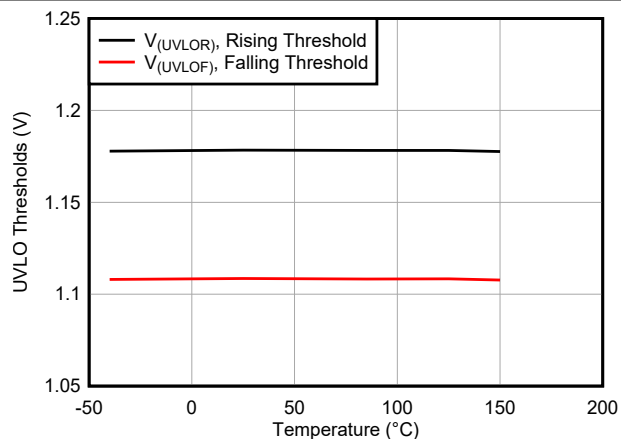
Figure 6-14. Input Supply UVLO Thresholds vs Temperature
