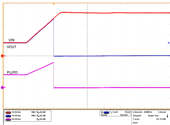
Figure 9-14. Overtvoltage Cutoff Response of TPS12110-Q1 at 36-V Level
