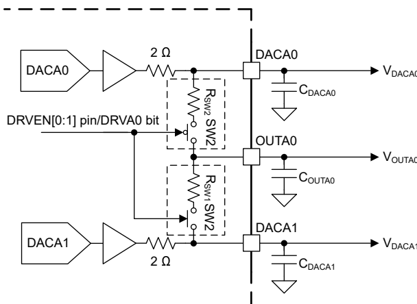
Figure 8-1. Switching Transients
