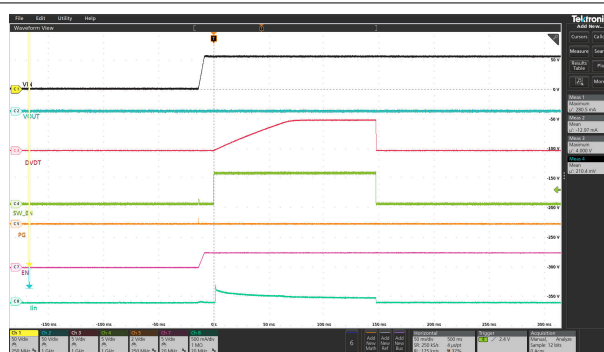
Figure 6-20. Overcurrent Protection Response (Circuit-Breaker)
