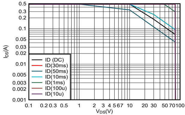
Figure 6-13. Allowed Operating Area (AOA) in Startup
