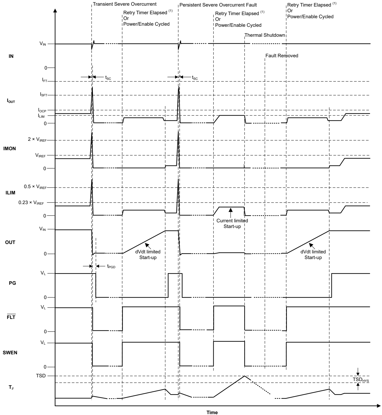
Figure 7-5. Short-Circuit Response
