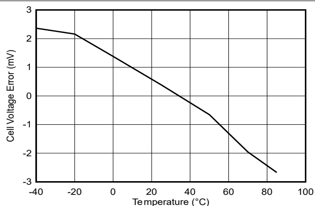
Figure 7-17. V_{CELL} Measurement Error at 3.5V vs. Temperature
