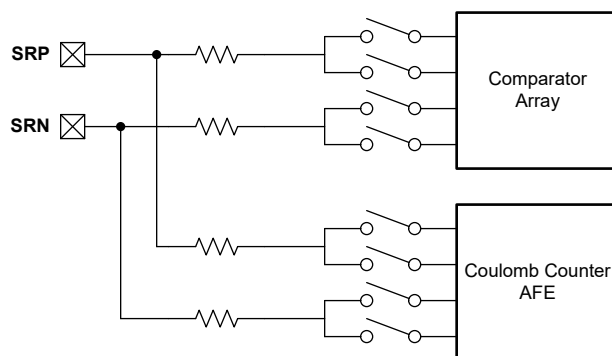
Figure 4-8. SRN, SRP Pins
