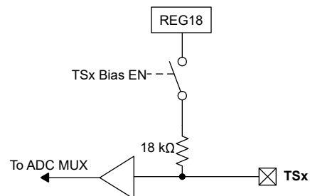
Figure 4-12. TSx Pins
