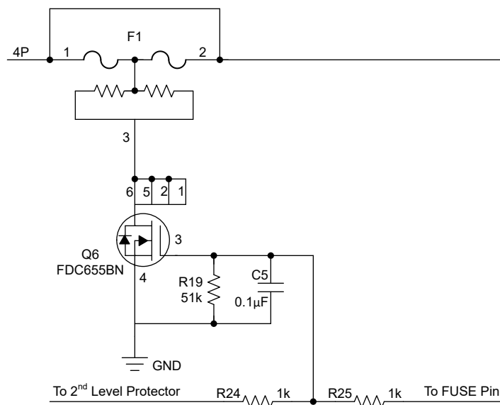
Figure 7-11. FUSE Circuit
