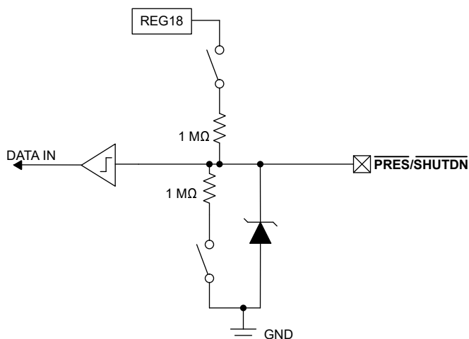
Figure 4-5. PRES/SHUTDN Pin
