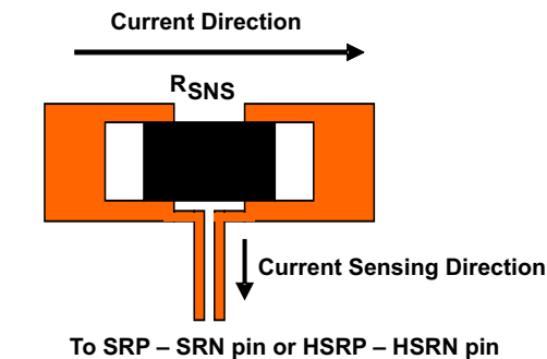
Figure 9-3. Sensing Resistor PCB Layout
