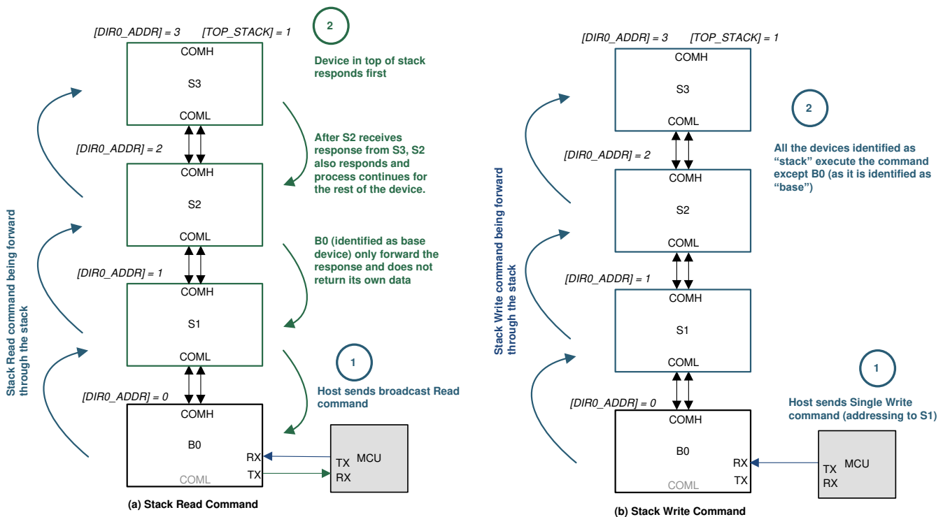
Figure 8-29. Stack Read/Write
