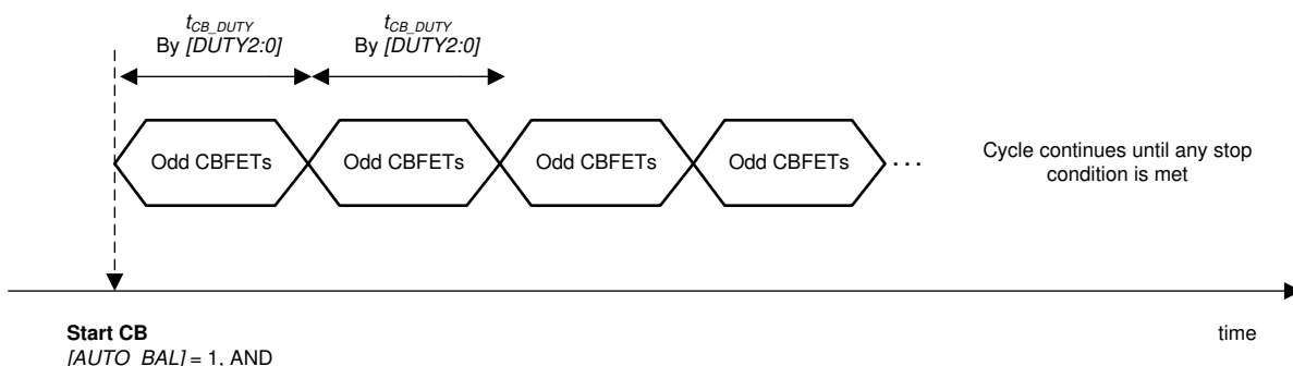
Figure 8-15. Auto Balancing Control, Example 2
