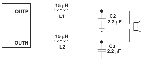
Figure 8-5. Typical LC Output Filter, Cutoff Frequency of 27 kHz, Speaker Impedance = 6 Ω
