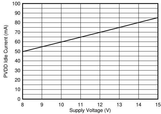
A. Load = 8 Ω Ferrite Bead Filter
