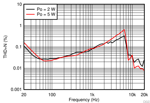
A. AVCC=PVCC = 12 V Load = 4 Ω 1SPW
