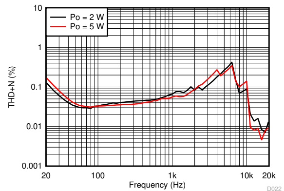
A. AVCC=PVCC = 12 V Load = 8 Ω 1SPW
