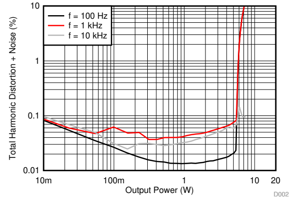
Figure 6-2. THD+N vs Power (BTL)
