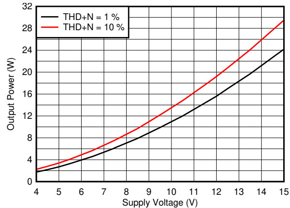
Figure 6-29. Output Power vs Supply Voltage, 4 Ω
