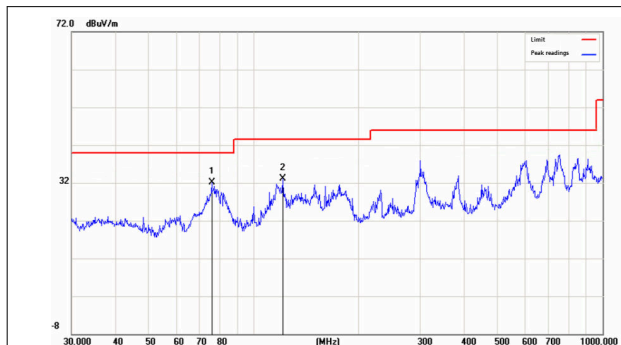
Figure 8-6. Radiated Emission - Horizontal
