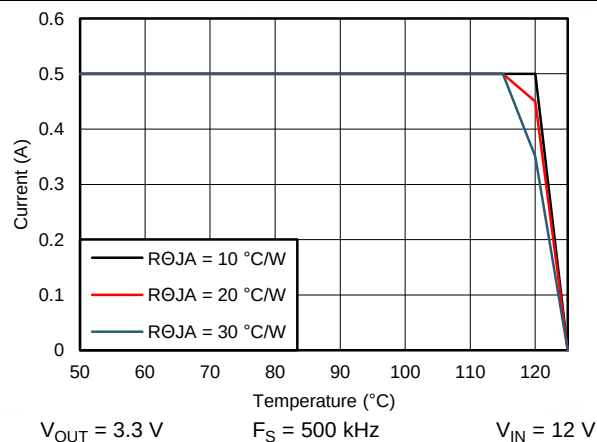
Figure 58. Derating Curve
