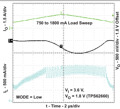
Figure 38. Overcurrent Fault Operation
