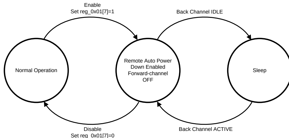
Figure 16. Remote Auto Power Down Sleep/Wake Cycle
