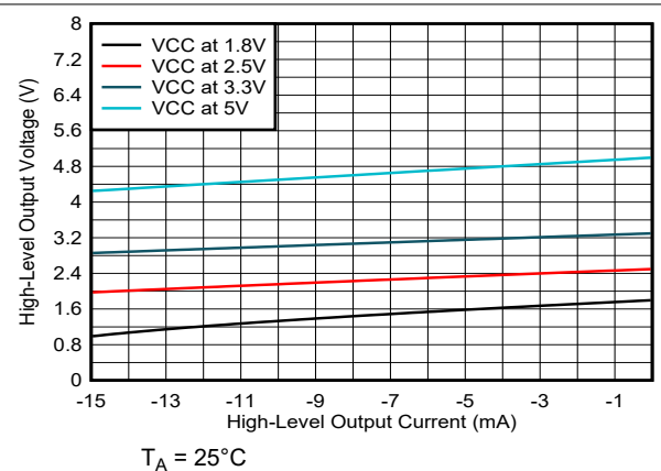
Figure 5-5. High-Level Output Voltage vs High-level Output Current
