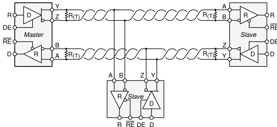
Figure 9-1. Half-Duplex Transceiver Configurations
