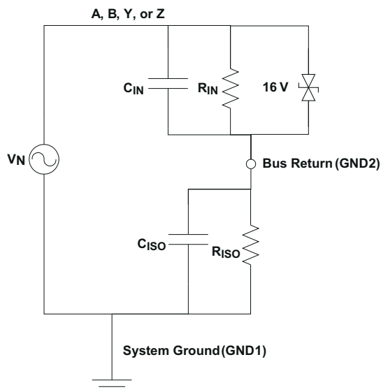
Figure 9-3. Noise Model
