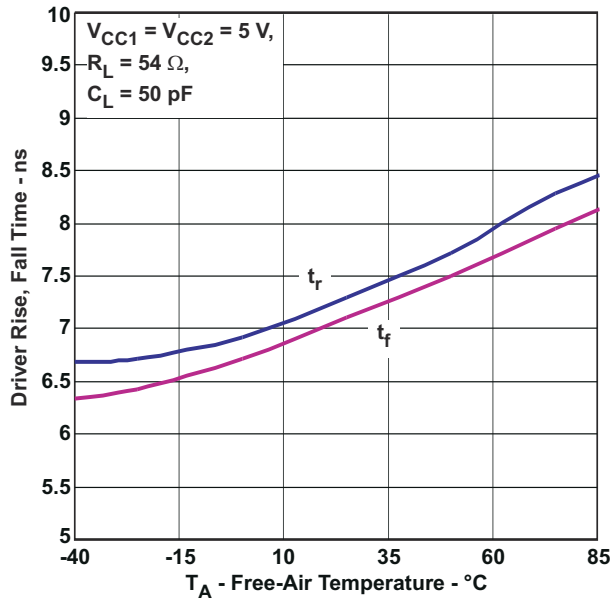
Figure 6-8. Driver Rise, Fall Time vs Free-Air Temperature
