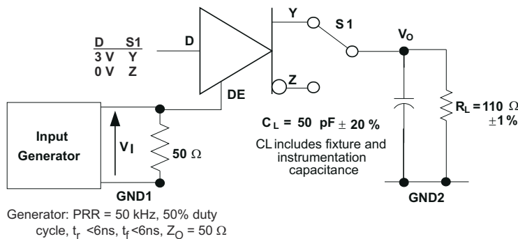
Figure 7-5. Driver High-Level Output Enable and Disable Time Test Circuit and Voltage Waveforms
