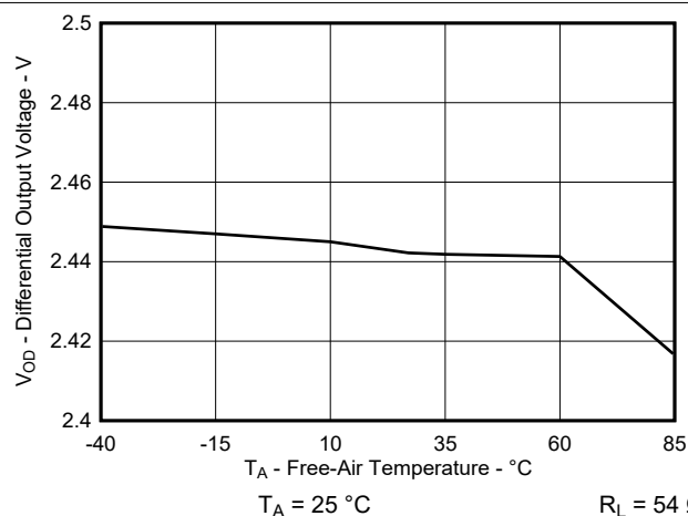
Figure 6-16. Differential Output Voltage vs Free-Air Temperature
