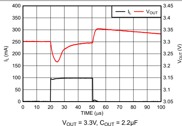
Figure 5-15. Load Transient Response (New Chip)
