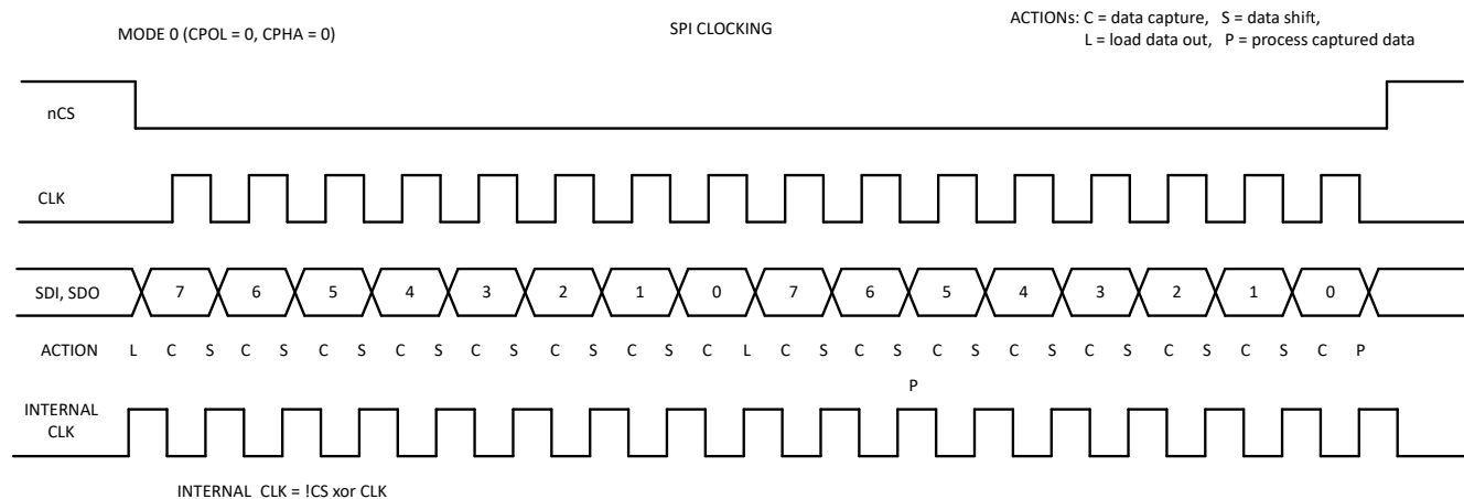
Figure 8-54. SPI Clocking
