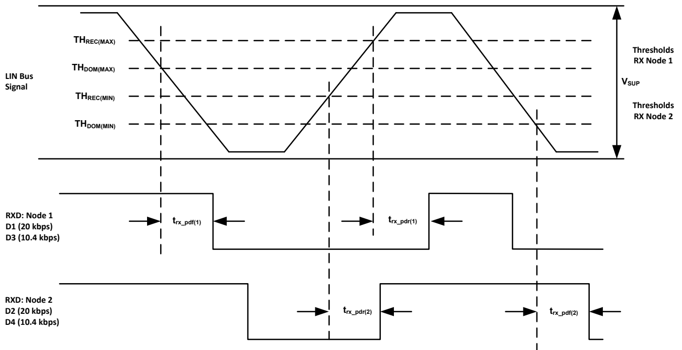
Figure 7-4. Propagation Delay
