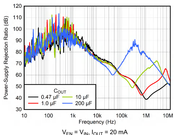
Figure 6-36. PSRR vs Frequency and C_{OUT}
