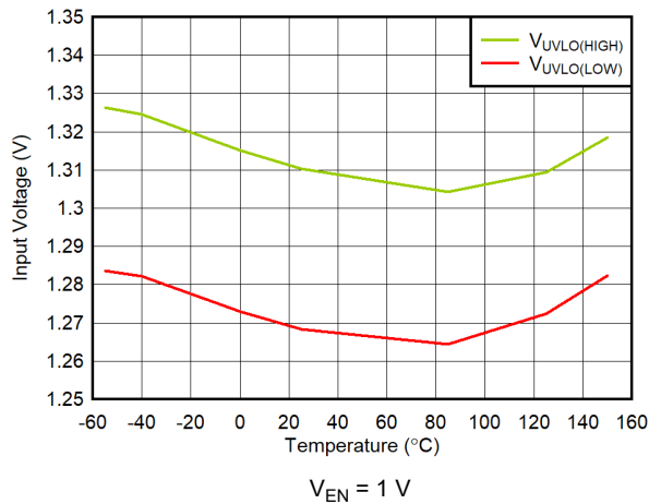
Figure 6-19. V_{IN} UVLO Threshold vs Temperature
