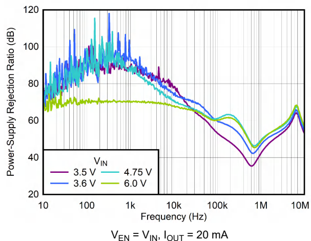
Figure 6-34. PSRR vs Frequency and V_{IN}
