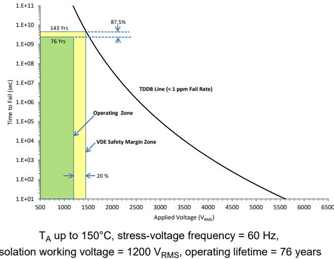
Figure 6-4. Reinforced Isolation Capacitor Lifetime Projection
