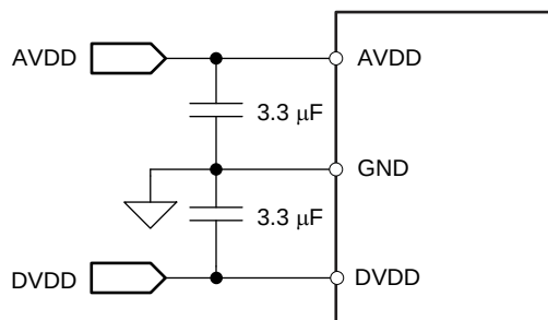
Figure 41. Power-Supply Decoupling
