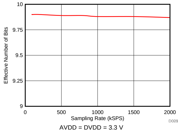
Figure 26. ENOB vs Sampling Rate
