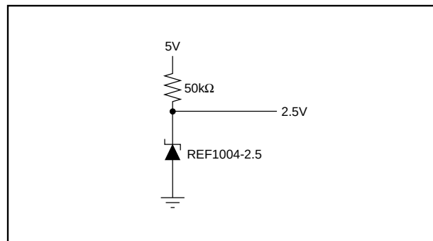
FIGURE 4. 2.5V Reference.
