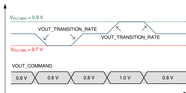
Figure 7-30. VOUT_MIN_MAX example
