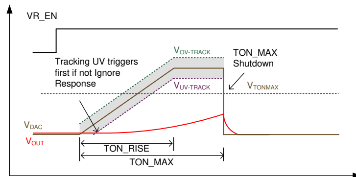
Figure 7-29. TON_MAX fault
