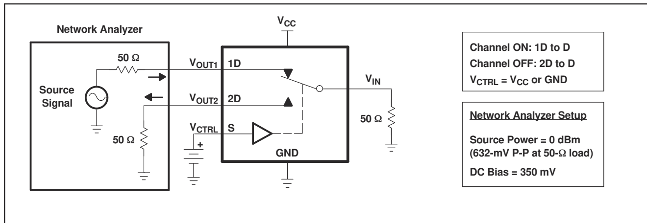
Figure 6-3. Crosstalk ( X_{TALK} )
