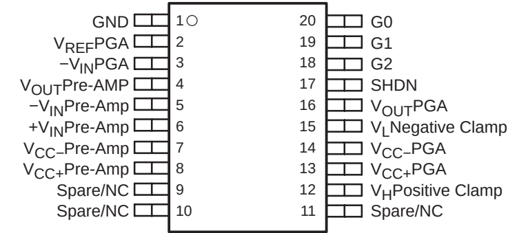
THS7001 PWP PACKAGE (TOP VIEW)
