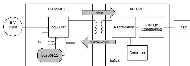
Simplified Schematic
