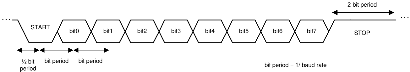
Figure 9-25. UART Response Frame with Two STOP Bits
