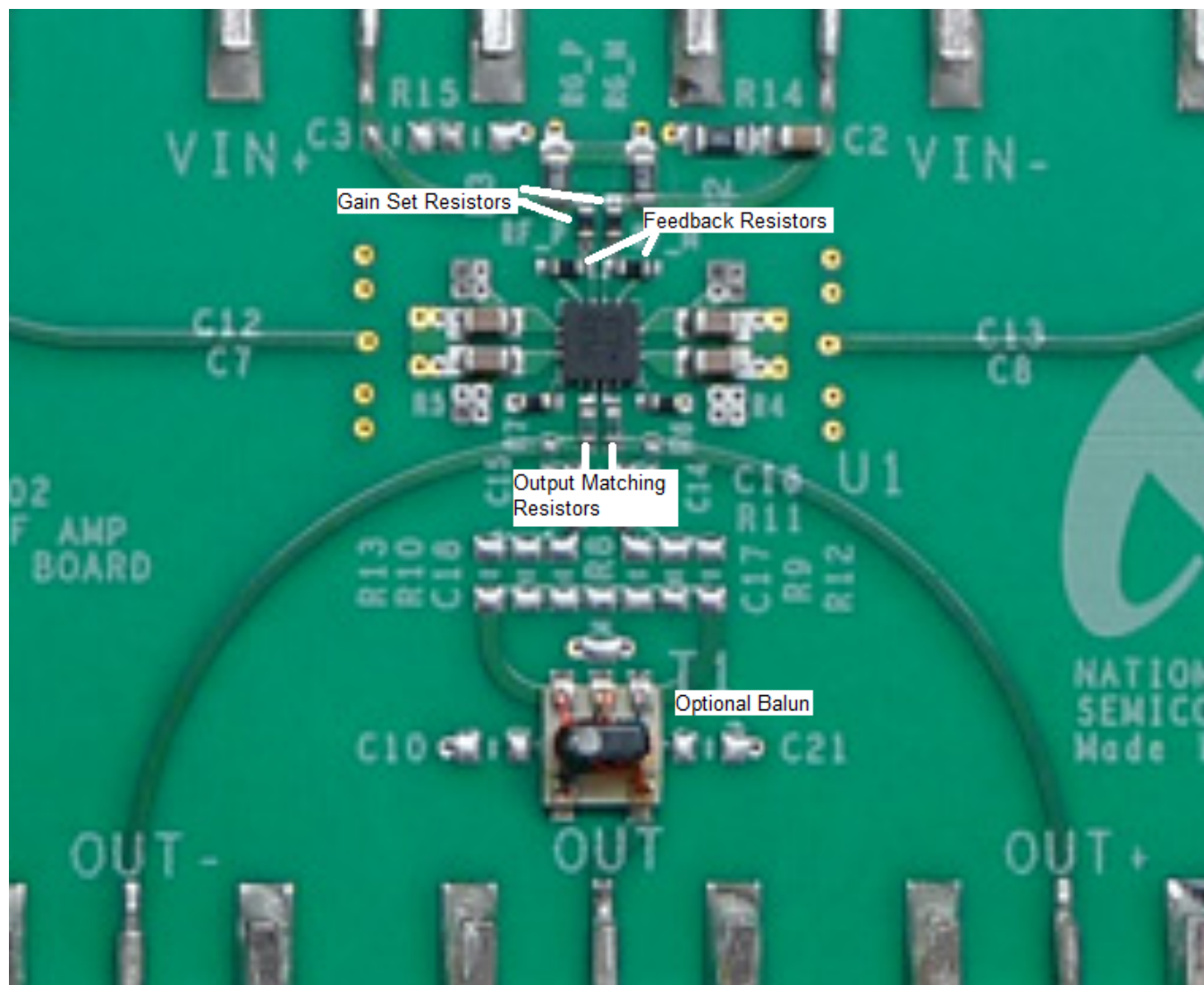
Figure 38. Layout Schematic
