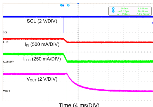
Mode bits (Reg 0x01 bit[1:0]) = 00 (Standby Mode)
