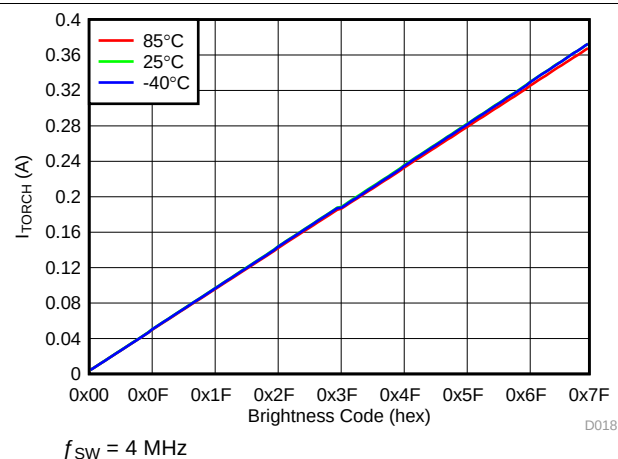
Figure 19. LED Torch Current vs Brightness Code
