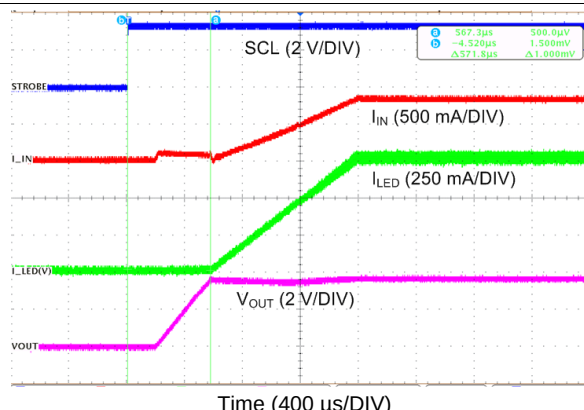
Time (400 \mu\text{s}/\text{DIV} ) STROBE Enabled (Reg 0x01 bit[2] = 1)
