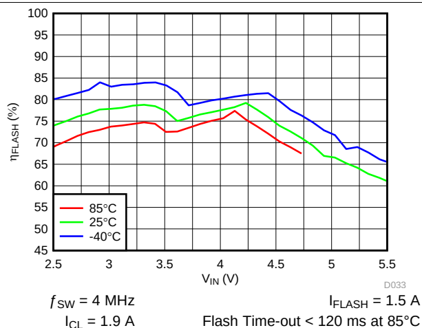
Figure 43. LED Flash Efficiency vs Input Voltage
