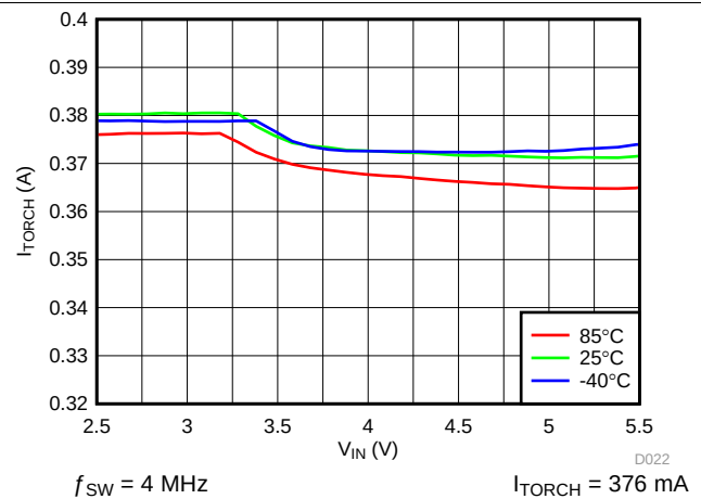
Figure 23. LED Torch Current vs Input Voltage
