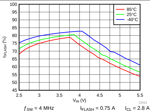
Figure 53. LED Flash Efficiency vs Input Voltage
