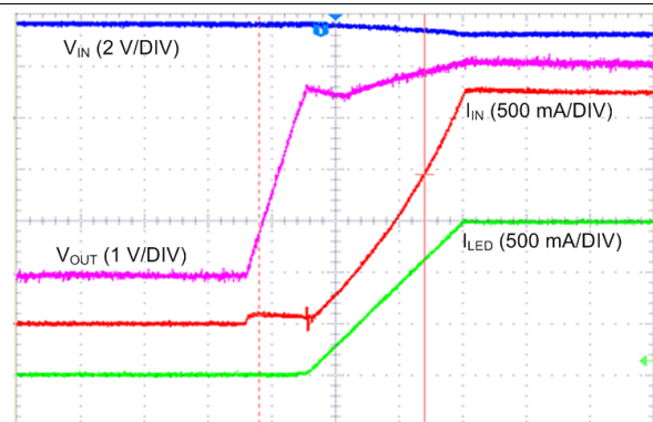
Figure 70. Boost I²C Torch
