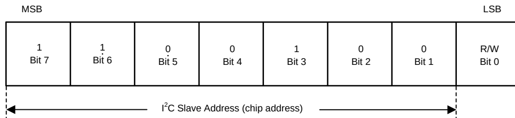
Figure 36. I 2 C-Compatible Chip Address
