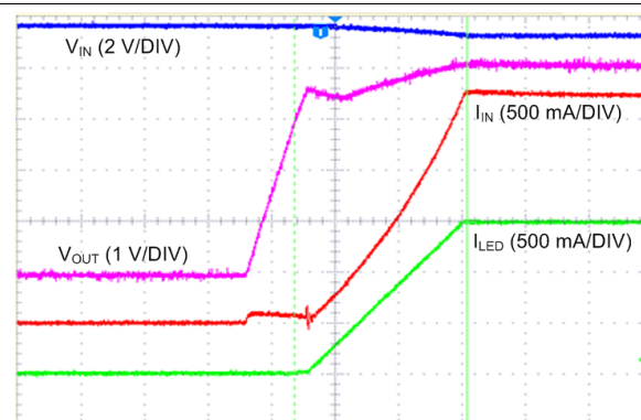
Figure 71. Boost I²C Flash
