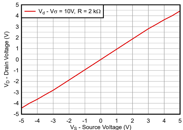
Figure 5-4. Source Voltage Input vs Drain Voltage Output
