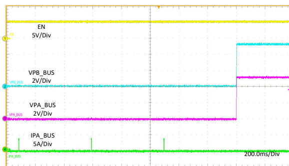
Figure 11-24. Short Circuit Recovery
