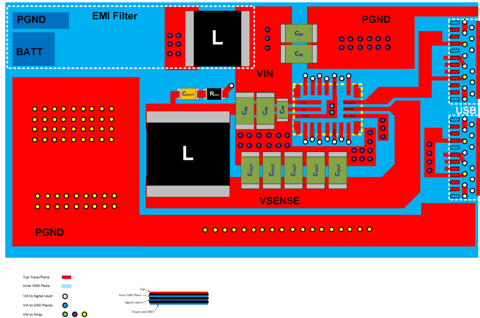
Figure 13-1. Layout Example
