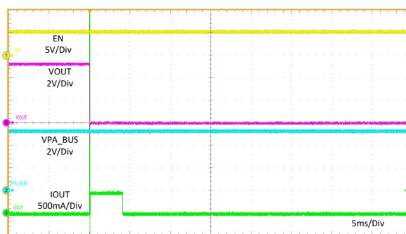
Figure 11-28. PA_CC2 Hot Short to GND
