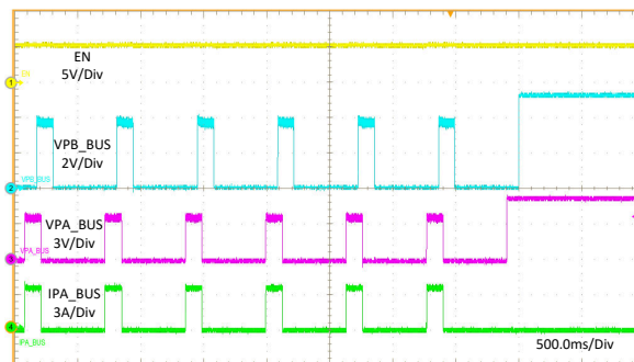
Figure 11-26. 1- \Omega Load Recovery
