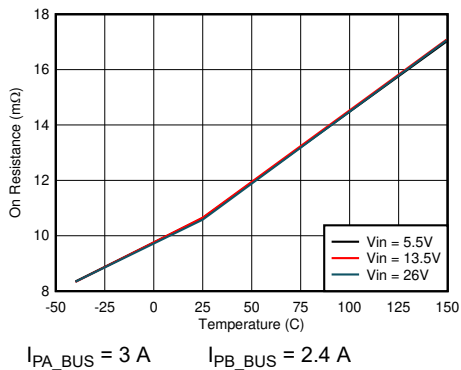
Figure 8-11. Low-side MOSFET on Resistance vs Junction Temperature
