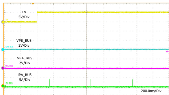
Figure 11-21. Rd Assert
