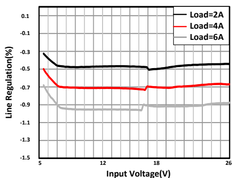
Figure 11-7. Line Regulation
