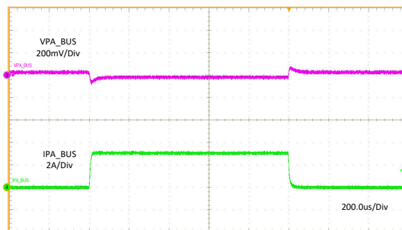
Figure 11-6. Load Regulation
