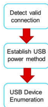
Figure 10-19. Flow of DFP-to-UFP Configuration
