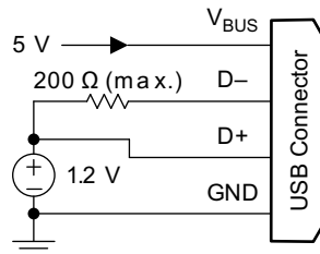
Figure 10-24. 1.2-V Mode
