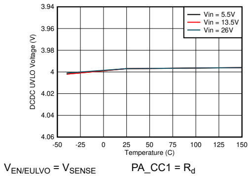
Figure 8-7. DCDC UVLO Threshold
