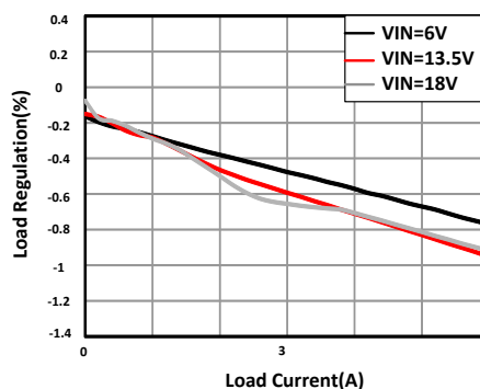
Figure 11-6. Load Regulation
