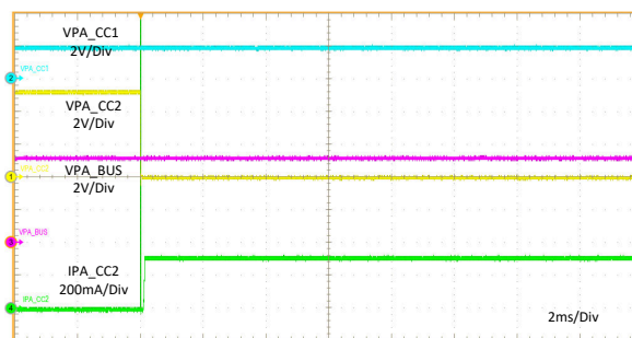
Figure 11-28. PA_CC2 Hot Short to GND
