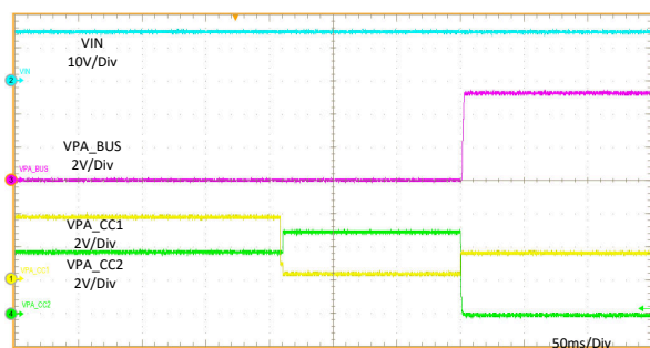
Figure 11-21. Rd Assert
